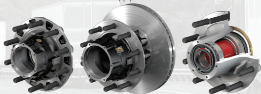
Iron Conventional Hub PreSet ® Iron Hub & Rotor PreSet Plus ® Aluminum Hub
